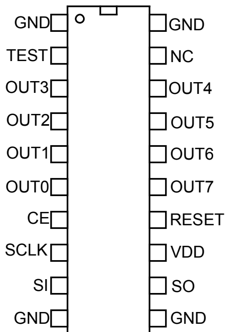
DIL 20
