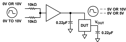
Figure 22. Turn-On/Transient Response Test Circuit
