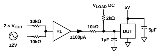
Figure 16. Output Impedance Test Circuit
