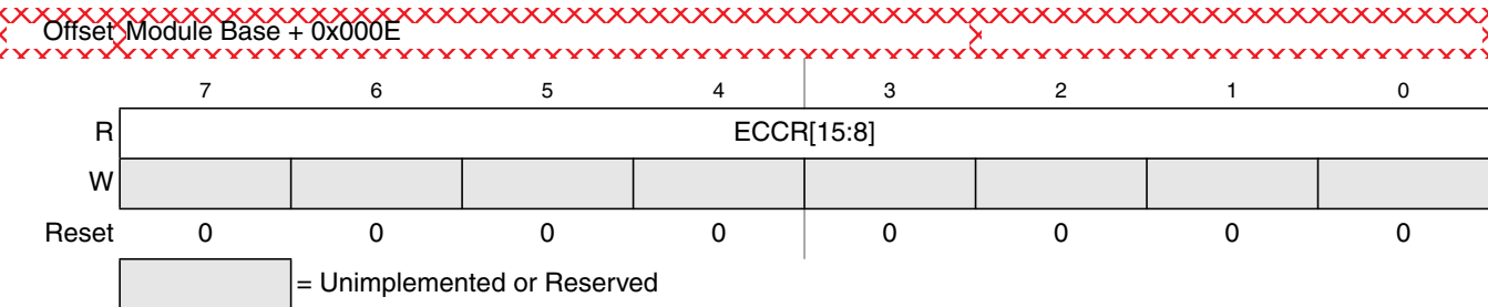
Figure 26-20. Flash ECC Error Results High Register (FECCRHI)
