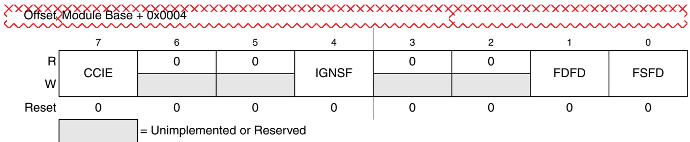
Figure 27-9. Flash Configuration Register (FCNFG)
