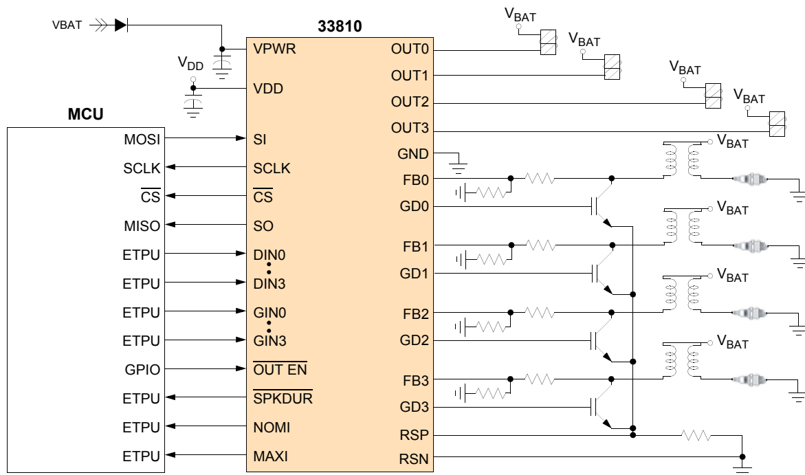
Figure 1. MC33810 Simplified Application Diagram
