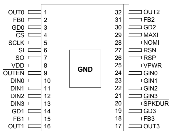
Figure 3. 33810 Pin Connections
