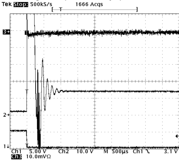
Figure 7. Open Secondary Spark Event
