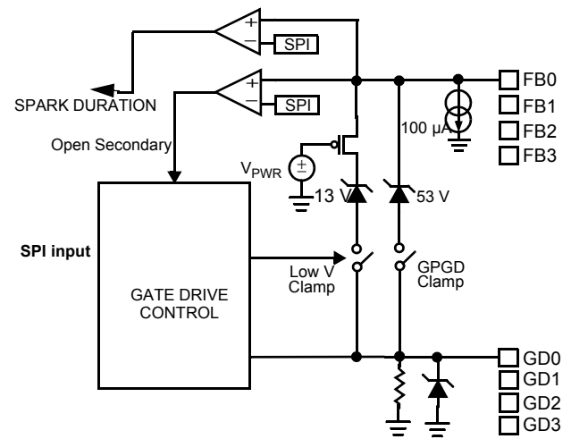
Figure 8. Low-voltage Clamp
