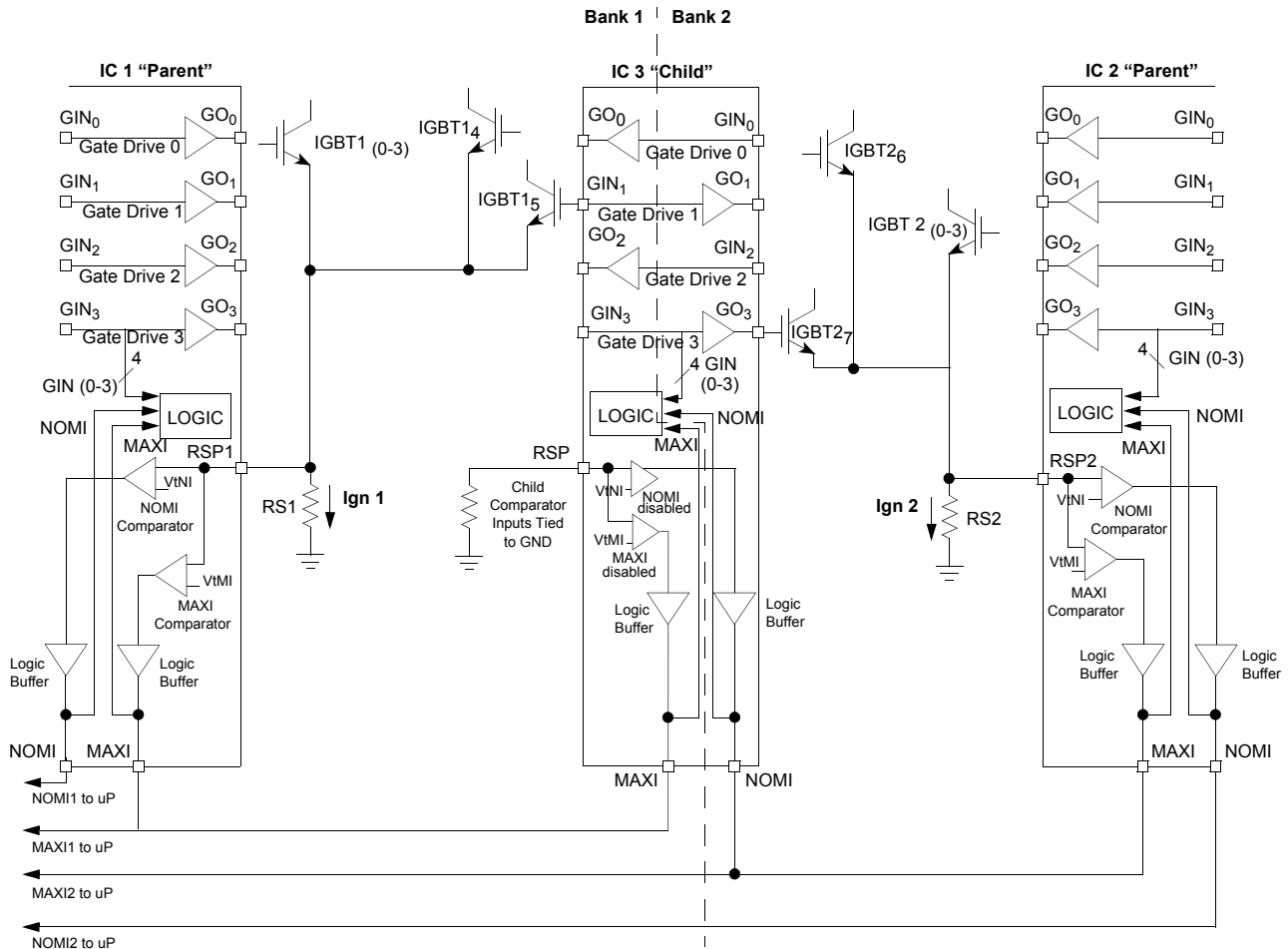
Figure 10. V10 Mode
