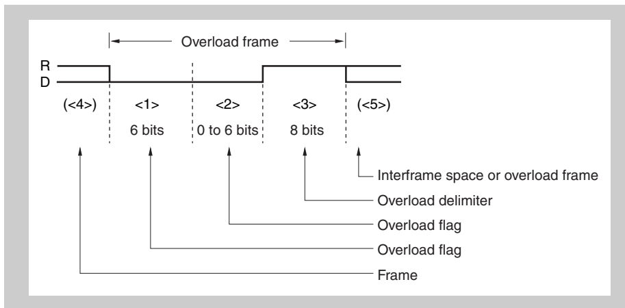
Figure 20-16 Overload frame
