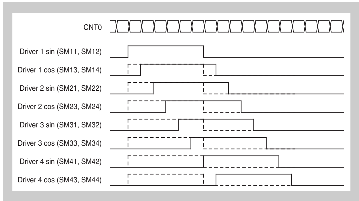
Figure 22-6 Output timing of signals SM11 to SM44
