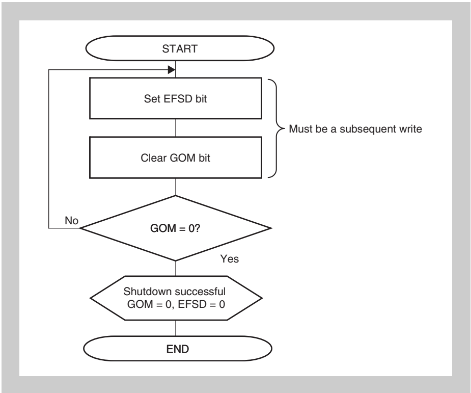
Figure 20-58 Forced shutdown process
