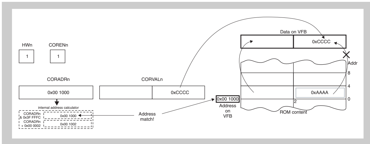
Figure 9-5 16-bit halfword aligned data replacement
