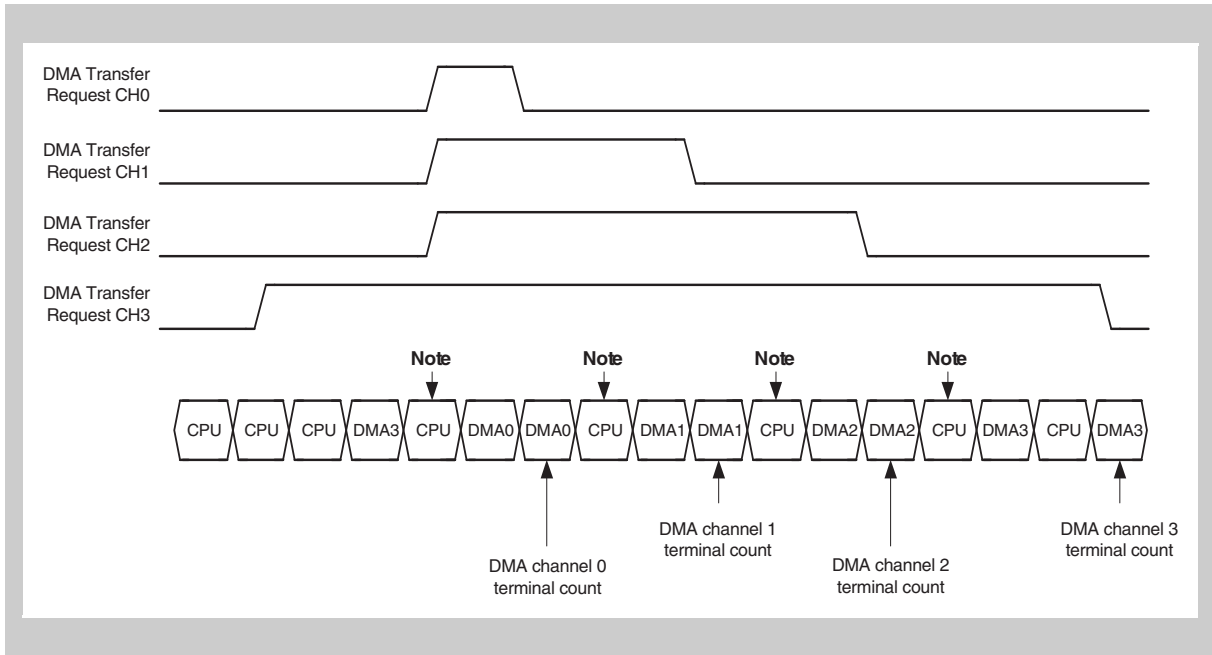
Figure 8-6 Single transfer example 2
