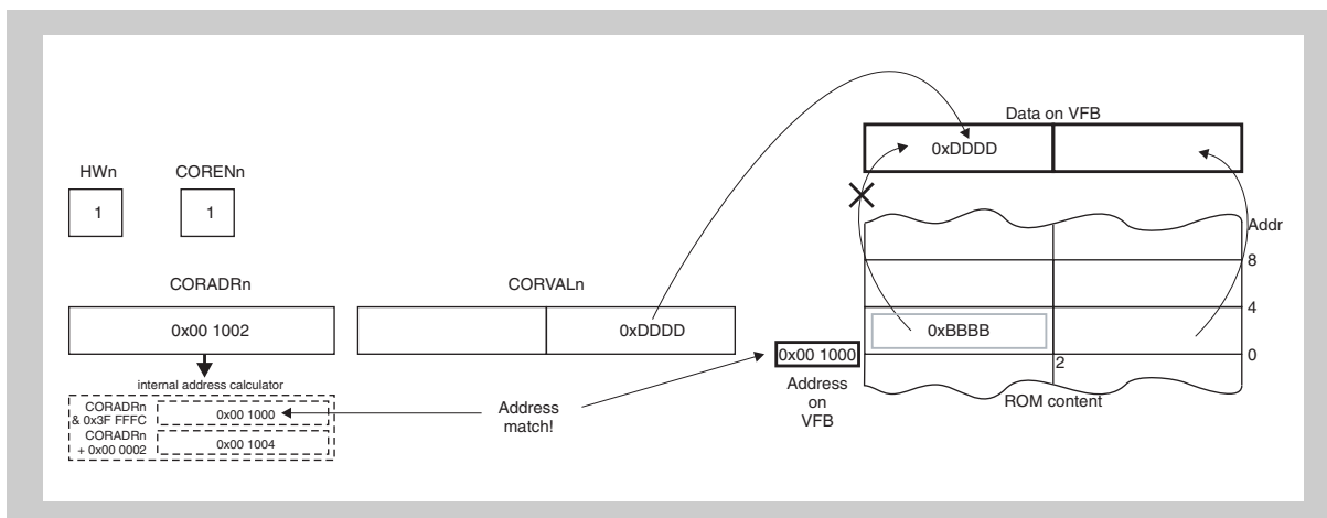
Figure 9-6 16-bit halfword unaligned data replacement
