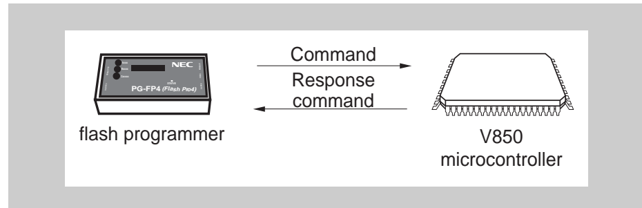
Figure 6-12 Communication commands
