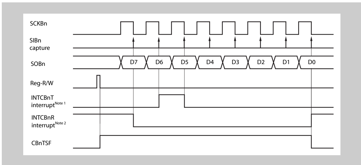
Figure 18-6 (ii) Communication type 3 (CBnCKP = 1, CBnDAP = 0)
