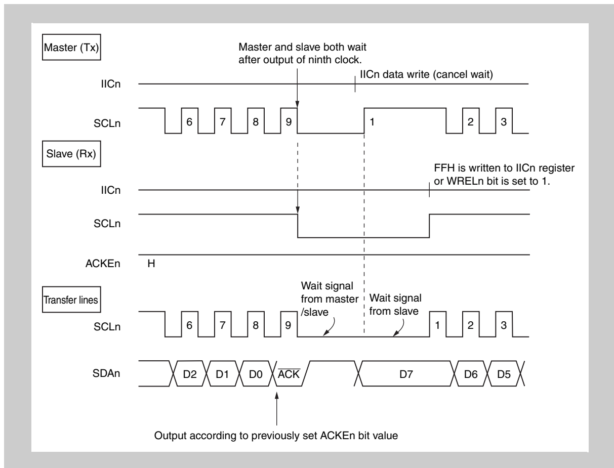
Figure 19-13 Wait signal (2/2)
