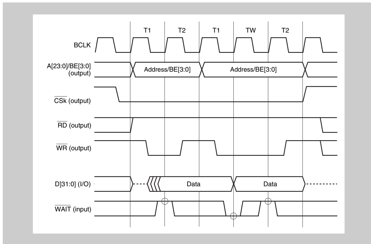
Figure 7-11 Timing: write data
