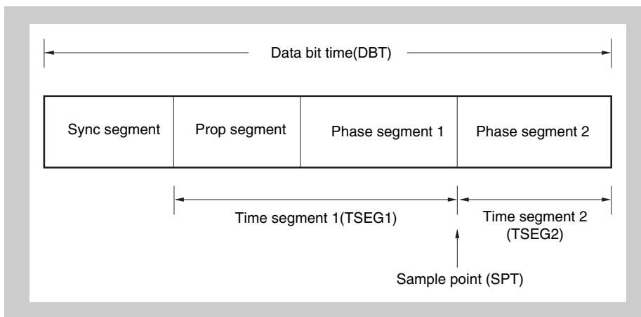
Figure 20-18 Segment setting
