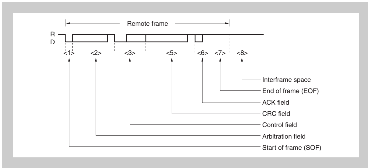
Figure 20-4 Remote frame
