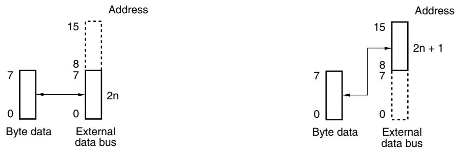
Figure 7-33 Left: Access to even address ( 2n ) Right: Access odd address ( 2n + 1 )
